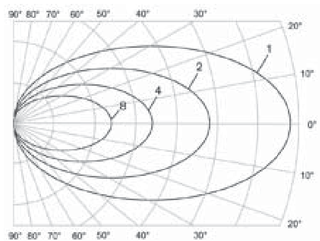
Polar diagram of the radiation pattern for 1, 2, 4 & 8 carriers
