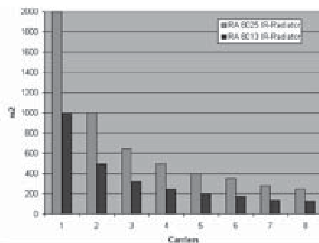
Total coverage area of RA 6013 & RA 6025 for 1 to 8 carriers
