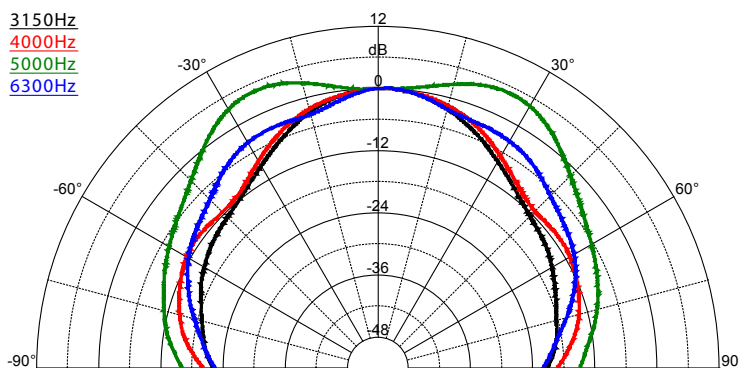
SAROS IC8T – Dispersion Pattern, 3150 Hz - 6300 Hz
